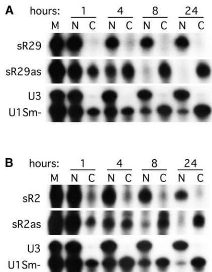
Figure 1. Archaeal Box C/D RNAs Are Stable and Retained in the Nucleus of Xenopus laevis Oocytes
