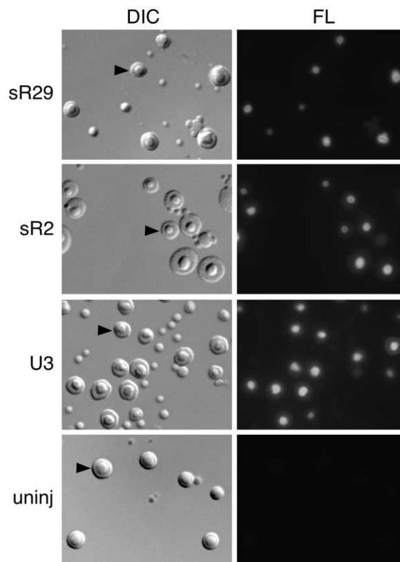
Figure 2. Targeting of Pyrococcus furiosus Box C/D RNAs to Xenopus laevis Oocyte Nucleoli
